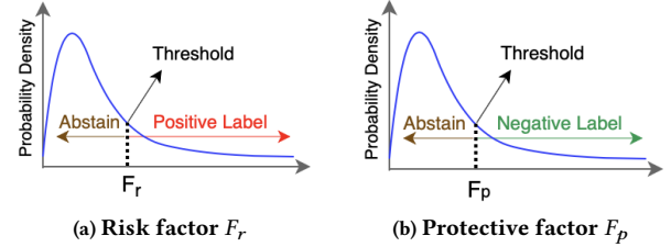
Figure 2: The proposed approach for defining labeling functions.
