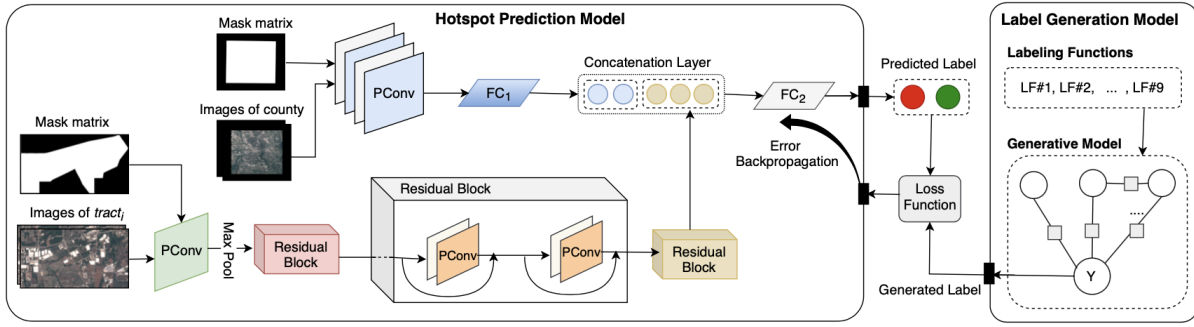
Figure 1: The architecture of WARNER.
