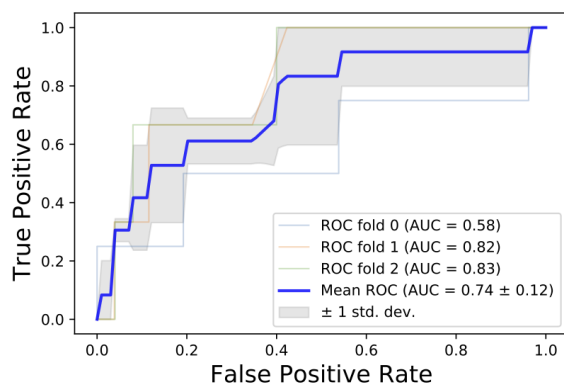
Figure 1: The ROC curve of our algorithm.
